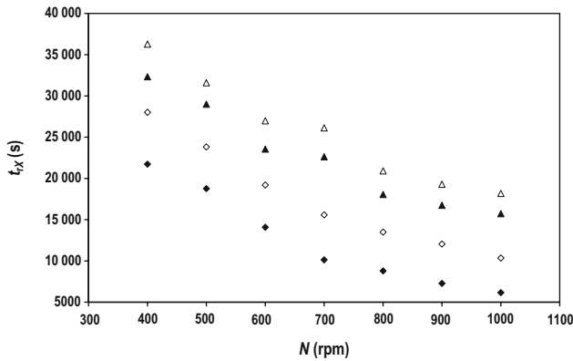
Figure 4. Rehydration time t_{xX} as a function of stirring speed N (rpm). \blacklozenge : X = 0.3 ; \diamond : X = 0.5 ; \blacktriangle : X = 0.7 ; \Delta : X = 0.9 . Fixed \phi and \theta values are equal to 4.8% (w/w) and 30 °C, respectively.
