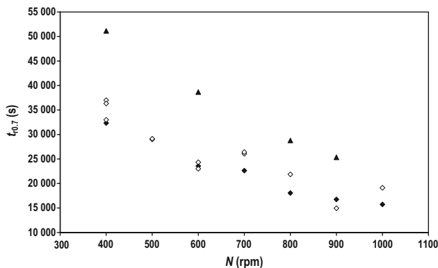
Figure 5. Rehydration time t_{r0.7} as a function of stirring speed N (rpm) for different solid-liquid concentrations \phi (w/w). \blacklozenge : \phi = 4.8\% ; \diamond : \phi = 8\% ; \blacktriangle : \phi = 12\% . Fixed \theta value is equal to 30\text{ }^{\circ}\text{C} .
