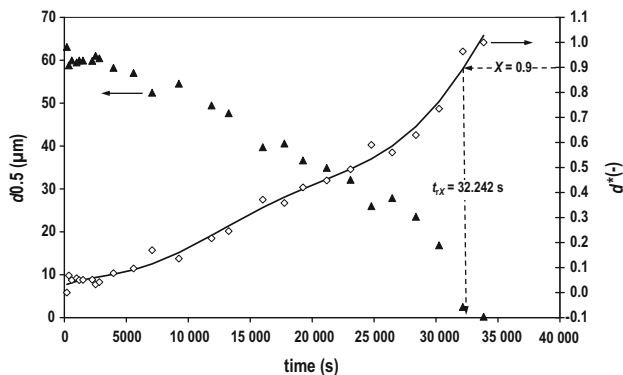
Figure 2. d_{0.5} and d^* as a function of time during rehydration of MCP at a concentration \phi of 8% (w/w), 30 °C and 500 rpm. \blacktriangle : d_{0.5} value; \diamond : corresponding d^* value calculated from equation (1); black line stands for polynomial model.
