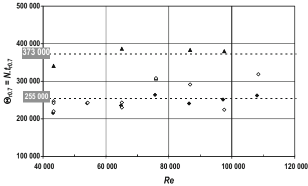
Figure 7. Rehydration time number \Theta_{r0.7} = N \cdot t_{r0.7} as a function of the Re number. \blacklozenge : \phi = 4.8\% ; \diamond : \phi = 8\% ; \blacktriangle : \phi = 12\% .
