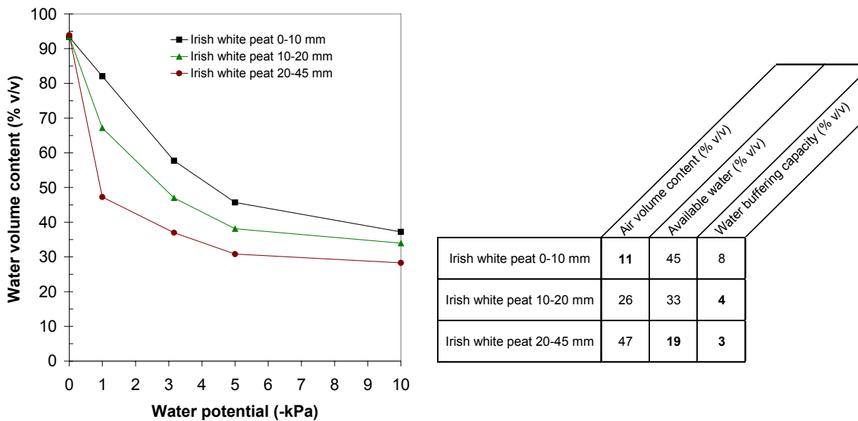
Figure 3. Examples of water retention curves of white Sphagnum peat with different particle size distributions.
