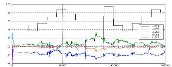
Fig.13. Humid duct model estimated parameters
