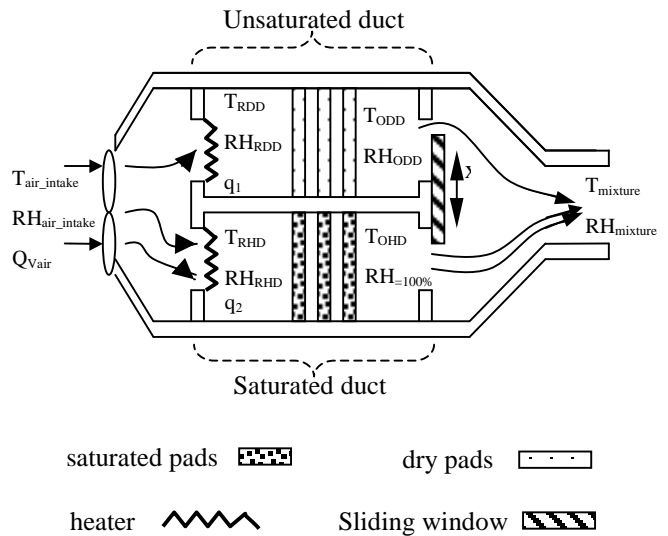
Fig. 9 Cross section view of the air-conditioning unit
