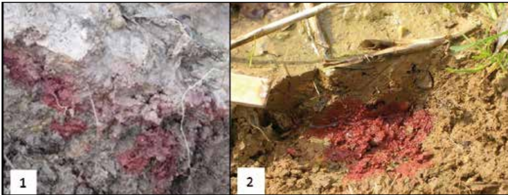
Figure 4 - 1 -Positive reaction over the compacted surface layer of a stagnosol; 2 -Positive reaction over the surface layer of a stagnic cambisol affected by a slaking crust.
