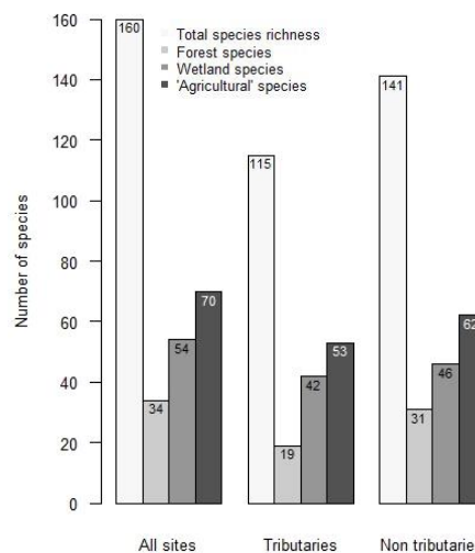
Fig. 2. Groups total richness – Sept. 2017
